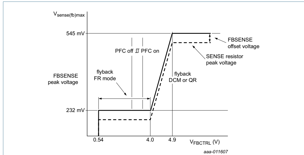
Fig 10. Flyback part peak current control
