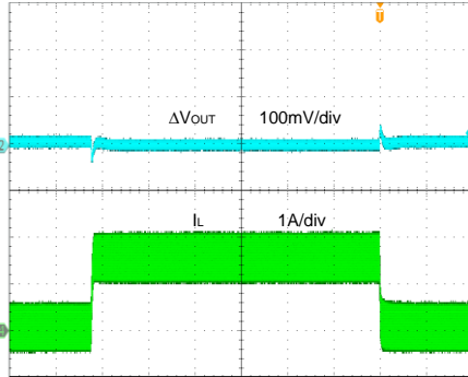
Load Transient
