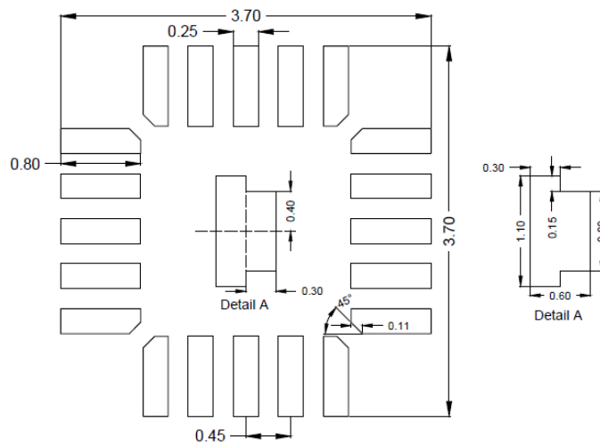
Recommended PCB layout (Reference only)
